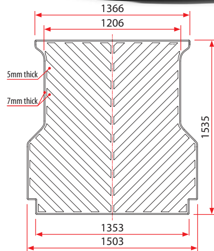
UTM-004 Mitsubishi MR-MQ Triton Bed Mat 2015-2023
