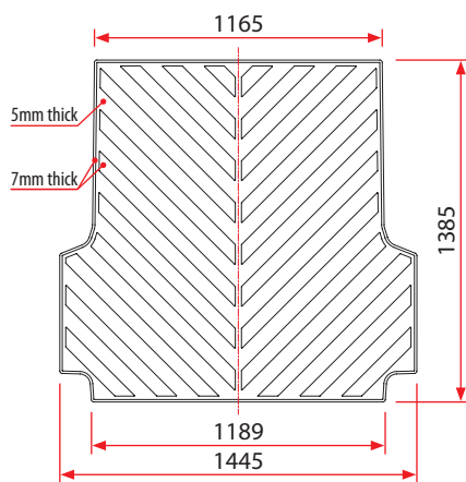
UTM-003 Toyota Hilux Bed Mat 2015-2023
